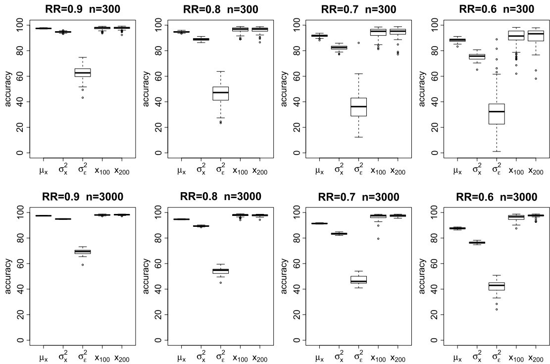
Fig. 2. Boxplots of parameter accuracies for the MFVB approximation applied to the nonparametric regression case corresponding to the simulation setting described in Section 5.2.
