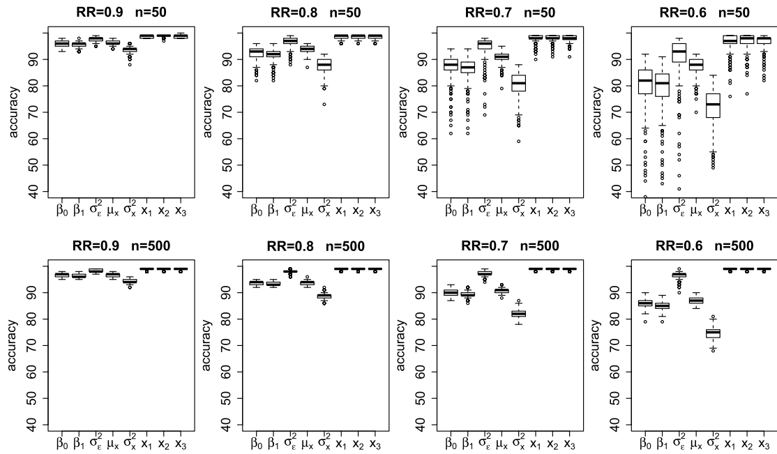
Fig. 1. Boxplots of parameter accuracies for the MFVB approximation applied to the simple linear regression case corresponding to the simulation setting described in Section 5.1.
