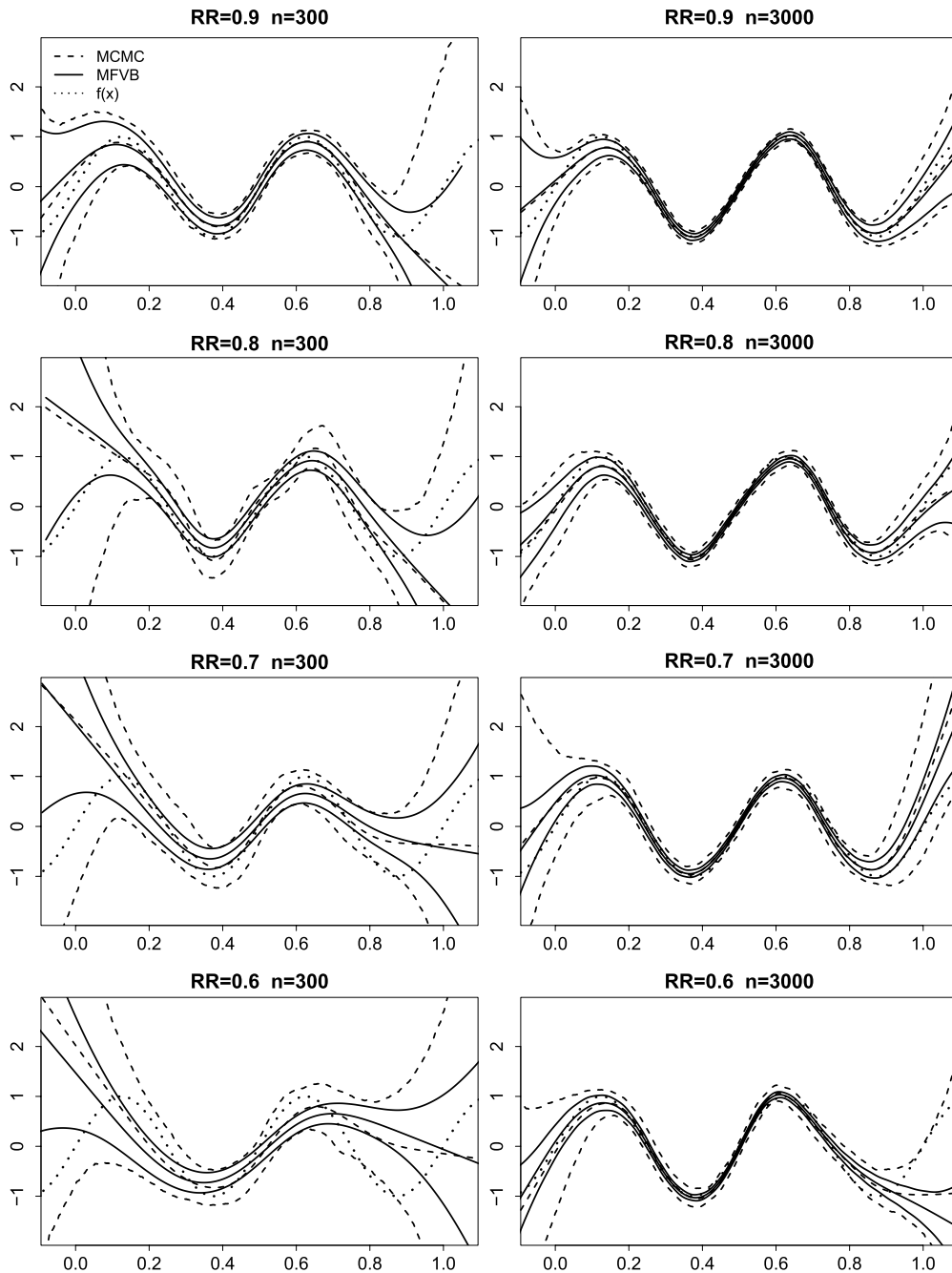
Fig. 3. Comparative plots of the approximated posterior distributions and the mean fitted functions with corresponding 95% credible sets for typical MFVB fits for simulated data described in Section 5.2 and for RR \in \{0.9, 0.8, 0.7, 0.6\} . MFVB estimates appear as solid lines whereas MCMC estimates appear as dashed lines.
