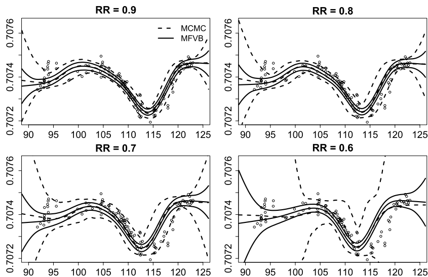
Fig. 4. Comparative plots of the approximated posterior distributions and the mean fitted functions with corresponding 95% credible sets for the Fossil dataset for RR \in \{0.9, 0.8, 0.7, 0.6\} . The x -axes correspond to date (in millions of years) and the y -axes correspond to strontium isotope levels. MFVB estimates appear as solid lines whereas MCMC estimates appear as dashed lines.
