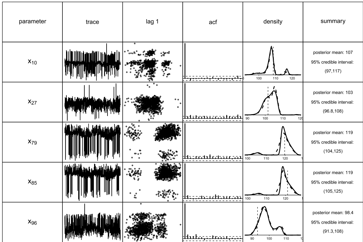
Fig. 6. Diagnostic plots for the MCMC analysis along with MFVB posterior density estimates for a random sample of x_i s (corresponding to indices: 10, 27, 79, 85 and 96). The columns are: missing predictor, trace plot of MCMC sample, plot of sample against 1-lagged sample, sample autocorrelation function, kernel estimates posterior density and basic numerical summaries. For the density column MCMC estimates appear as solid black lines whereas MFVB estimates appear as dashed lines.
